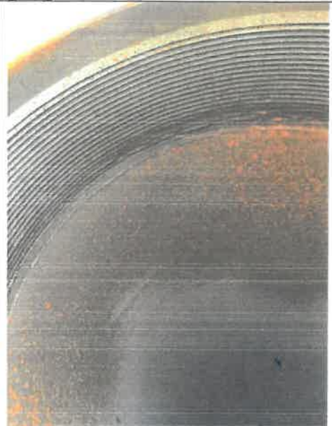
Lost threads in coupling
